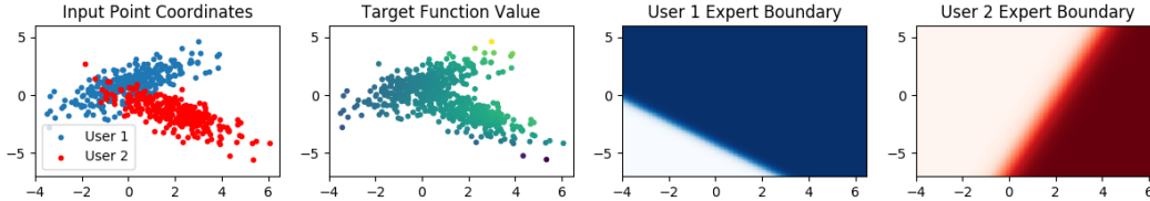
Figure 1: Visualizing the synthetic data experiment. Axes for all figures represent input values for x_1 and x_2 . Left to right: (a) x_1 and x_2 values of test data points sampled from distinct 2d Gaussians. (b) Target values of nonlinear function f(x_1, x_2) . (c) Values of the MoE gating function, \alpha_1(x_1, x_2) learned by User 1. In the darker region, the private domain expert is preferred, while the general model is preferred in the lighter region. (d) The gating function \alpha_2(x_1, x_2) of User 2, which uses the shared model in a different region than User 1.
