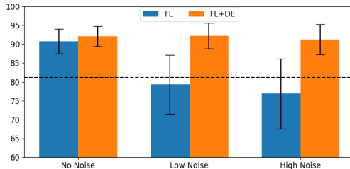
Figure 2: Classifier accuracy on the spam dataset (higher is better). FL and our system (FL+DE) are evaluated as gradient noise is increased (for differential privacy). The dashed horizontal line indicates domain-only baseline performance. Error bars show performance variance across users.
